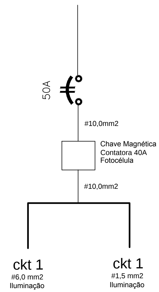
Diagrama Unifilar
